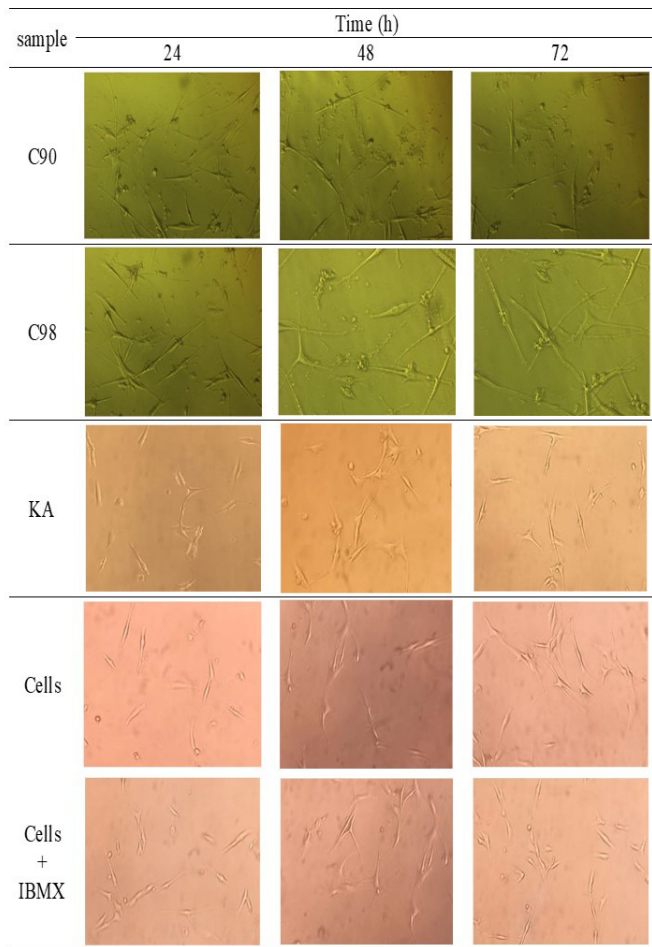
Figure 5. Morphological form of decreased extracellular melanin content from C90, C98, and KA at a concentration of 80 µg/ml.
