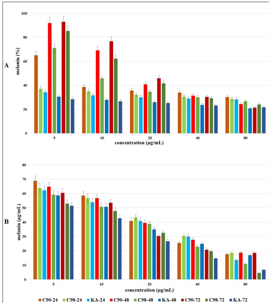
Figure 4. Effect of C90, C98, and KA on melanin content extracellular (A) and intracellular (B) in B16F0 cells at different concentrations (5, 10, 20, 40, and 80 µg/ml) with the test duration of 24, 48 and 72 hours. Error bars represent the standard deviation ( n = 3).
