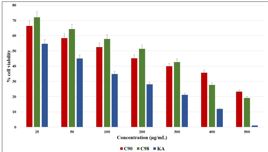
Figure 1. Cell viability assay using the MTT assay, B16F0 cells were treated with C90, C98, and KA at different concentrations (25, 50, 100, 200, 300, 400, and 500 µg/ml) in 72 hours. Error bars represent the standard deviation ( n = 4 ).
