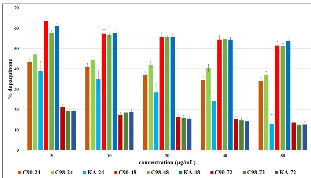
Figure 3. The reaction of the TYR enzyme to dopaquinone is a rate-limiting step in the melanogenesis of melanin formation.
