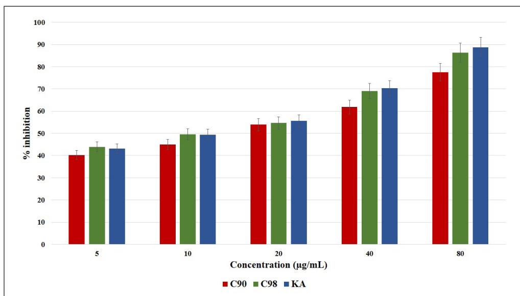
Figure 2. Percentage of inhibition of C90, C98, and KA on mushroom tyrosinase enzymes with different concentrations (5, 10, 20, 40, and 80 µg/ml). Error bars represent the standard deviation ( n = 3 ).
