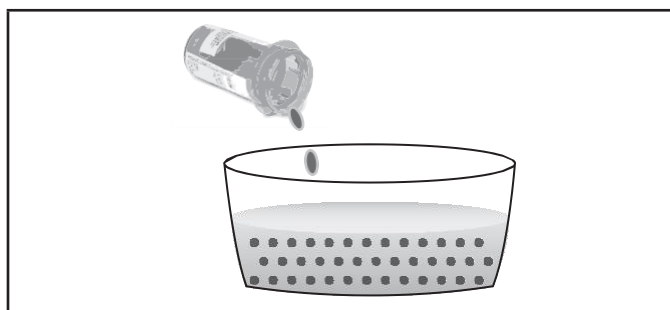
FIGURE 1-20. The volume of a tank can be determined from the amount of substance added and the resulting concentration.
